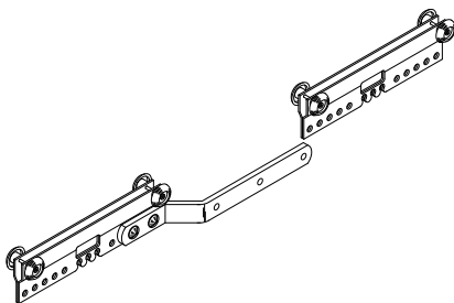
No. 5282 Master Carrier w/Arm Cannot be used on curved tracks.
