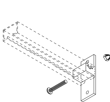
No. 5202 Wall Bracket
