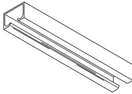
No. 5250 Track 6', 12', 16' and 20' Stock Lengths
