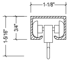
DIMENSION DRAWINGS
