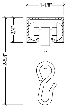
No. 5203 Ceiling Bracket
